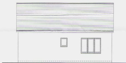
PROPOSED NORTH WEST ELEVATION
